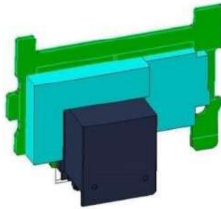
Figure 24. R3 Paddle (routes PCIe lanes to front backplane for additional NVMe)
