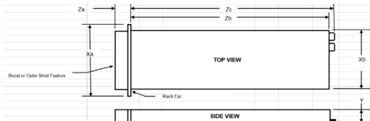
Figure 32. Chassis dimensions
